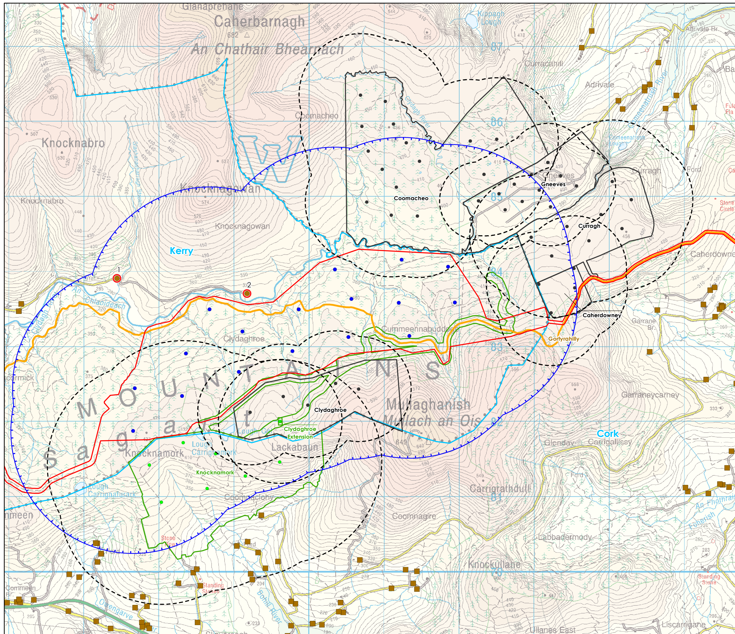
Figure 15-2a Cumulative shadow flicker extents and Maximum Rotor Diameter
